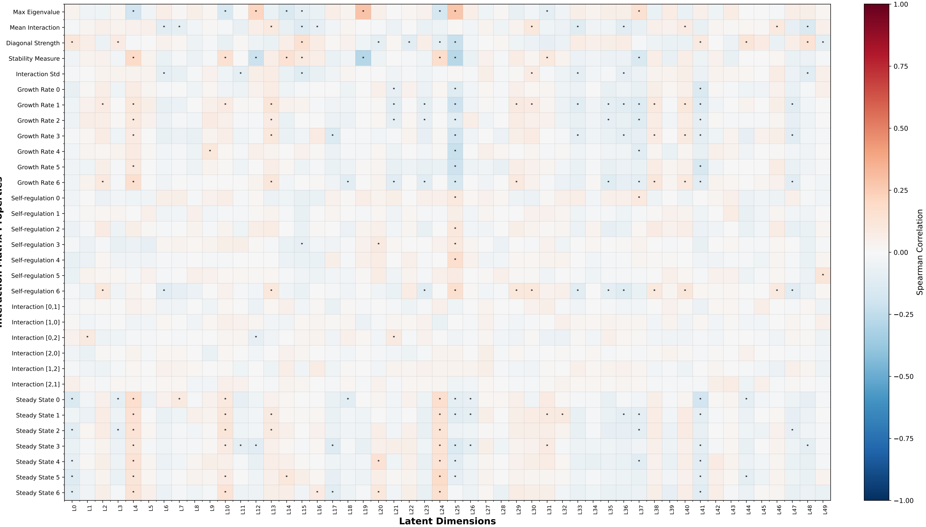
Correlation Heatmap: 50 Latent Dimensions vs GLV Properties (Spearman correlation, * indicates p<0.01)
